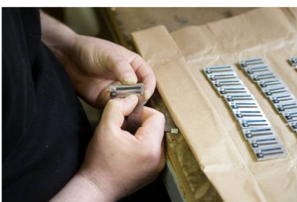
ADJUSTMENT OF THE TONGUES OF THE REEDS
